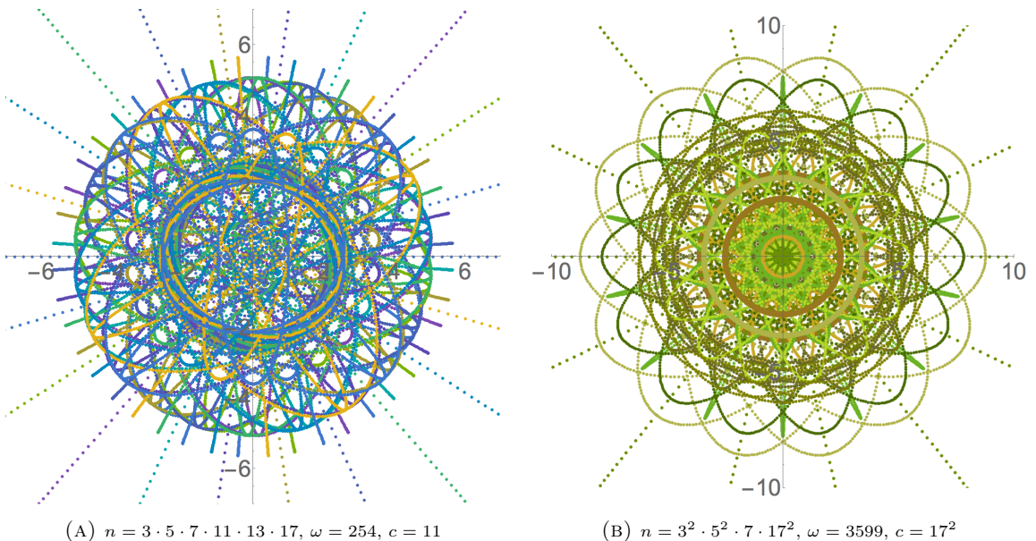
FIGURE 4. Atoms — Images of cyclic supercharacters correspond to sets of Gaussian periods. For notation and terminology, see Section 3.
