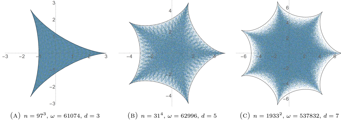
FIGURE 9. Certain cyclic supercharacters fill out regions bounded by hypocycloids , outlined in black (see Proposition 1).
