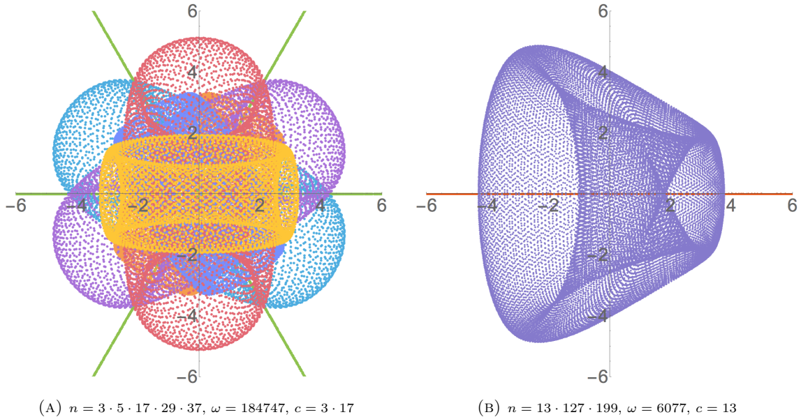
FIGURE 2. Disco ball and loudspeaker — Images of cyclic supercharacters correspond to sets of Gaussian periods. For notation and terminology, see Section 3.
