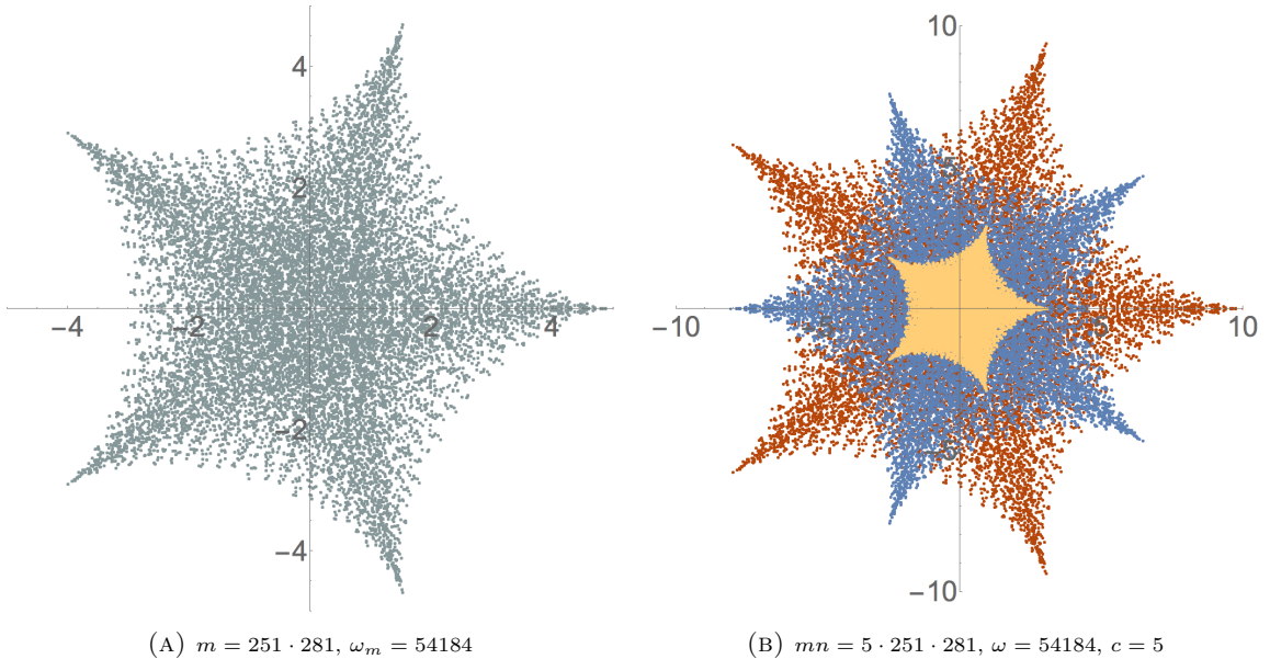
FIGURE 6. The image on the right is the product set of the image on the left and the image \{2, \frac{1}{2}(\pm\sqrt{5} - 1)\} , as in (3).
