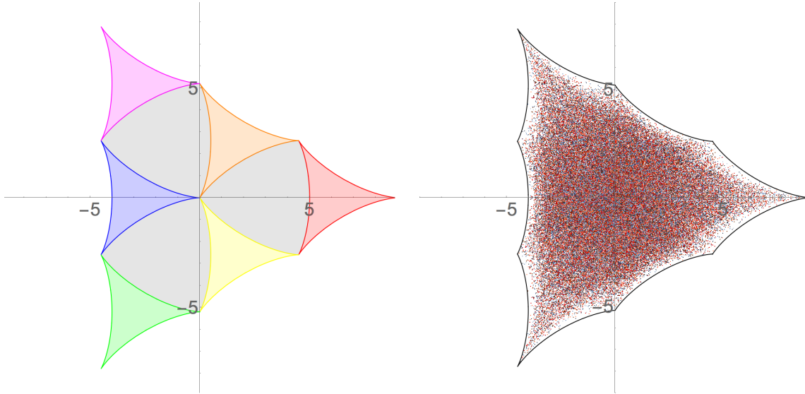
(A) A geometric interpretation of H_3 + H_3 + H_3
