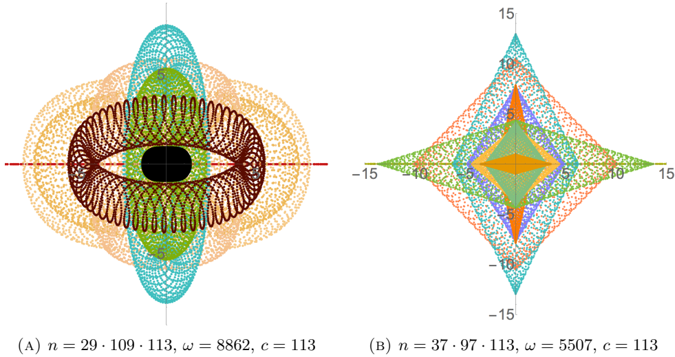
FIGURE 1. Eye and jewel — Images of cyclic supercharacters correspond to sets of Gaussian periods. For notation and terminology, see Section 3.
