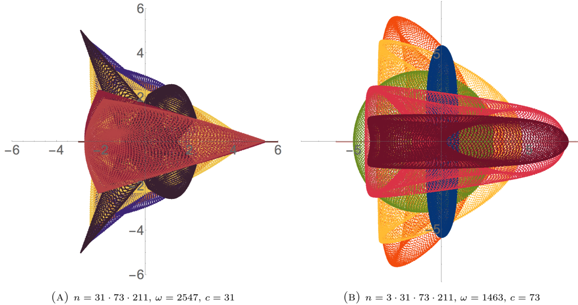
FIGURE 5. Bird and spacecraft — images of cyclic supercharacters.
