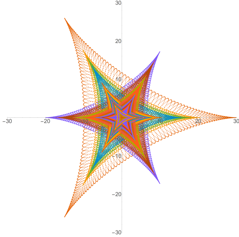
FIGURE 7. n = 127^2 \cdot 401 , \omega = 6085605 , c = 401
