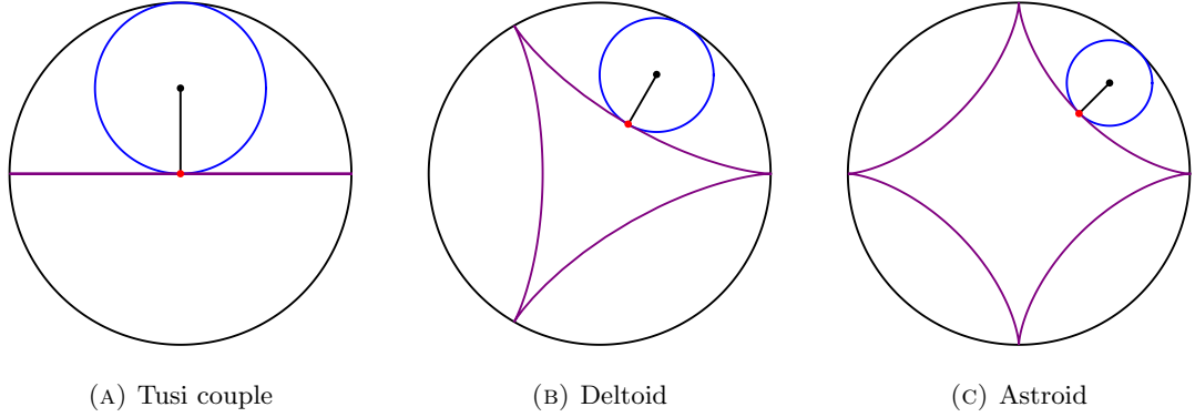
FIGURE 10. Circles of radius 1 trace out hypocycloids as they roll within circles of radii (from left to right) 2, 3, and 4.
