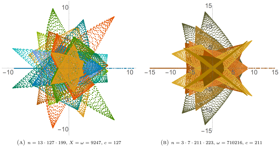
FIGURE 3. Mite and moth — Images of cyclic supercharacters correspond to sets of Gaussian periods. For notation and terminology, see Section 3.
